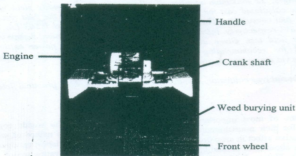
Plate 1. Newly designed burial type lowland power cultivator.
